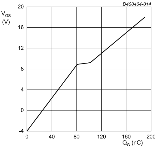
I_{DS} = 75\text{ A} ; I_{GS} = 0.1\text{ mA} ; V_{DS} = 400\text{ V} ; T_j = 25\text{ }^{\circ}\text{C} Fig. 14. Gate-source voltage as a function of gate charge; typical values
