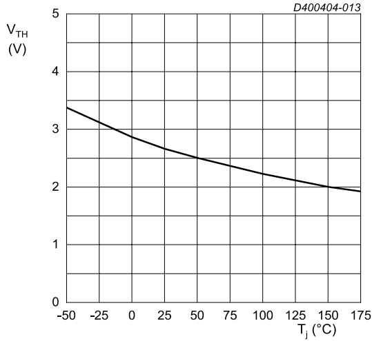
V_{DS} = V_{GS} ; I_{DS} = 18\text{ mA} Fig. 13. Threshold voltage as a function of junction temperature
